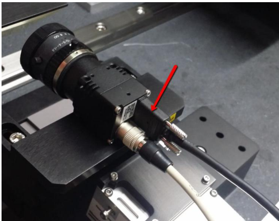
Figure 8 PSP 2 Camera Cable
