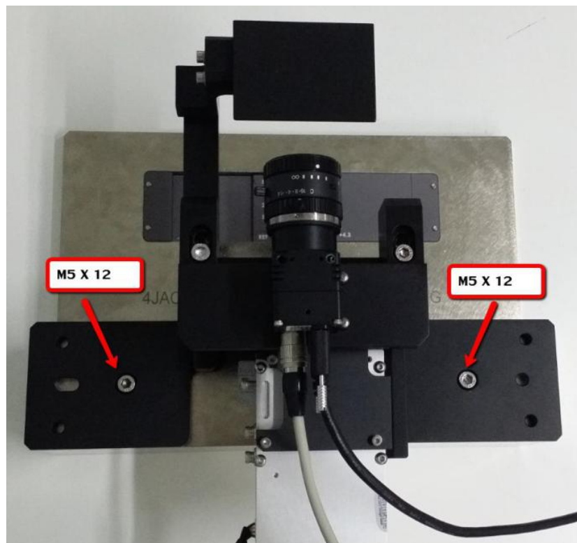
Figure 2 S2EX OFFLINE JIG ASSEMBLY
