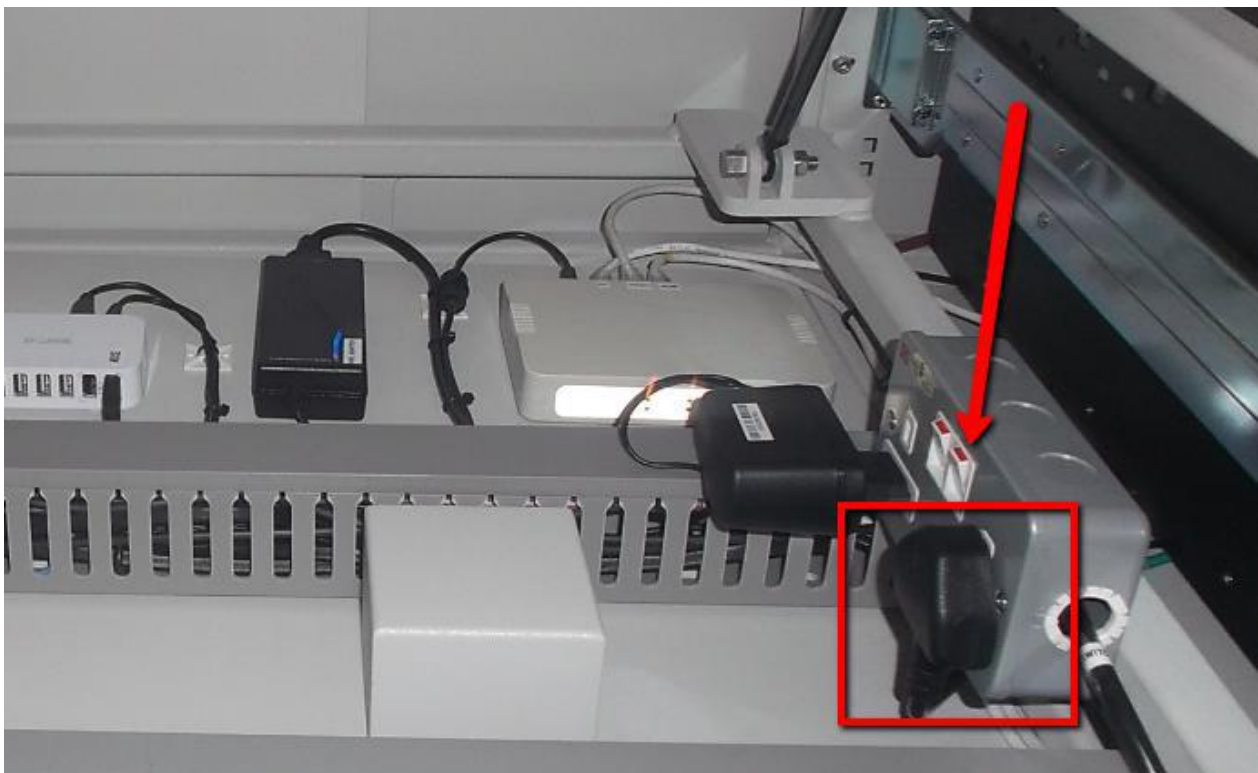
Figure 4 3 PIN PLUG POWER SWITCH
