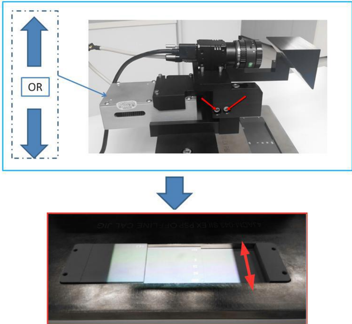
Figure 38 White Light Projection Coverage Area
