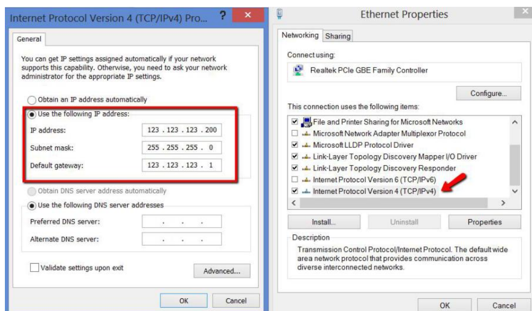
Figure 15 EBLE (PROJECTOR IP PORT) SETTING
