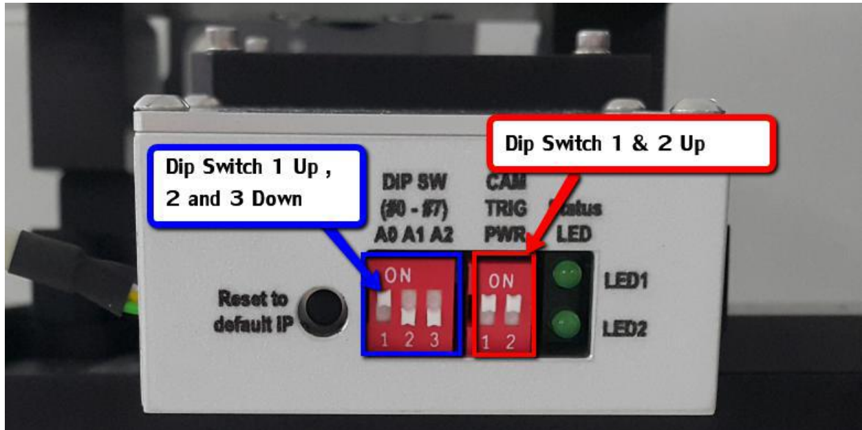
Figure 1 Rear Projector IP DIP SWITCH CONFIGURATION
