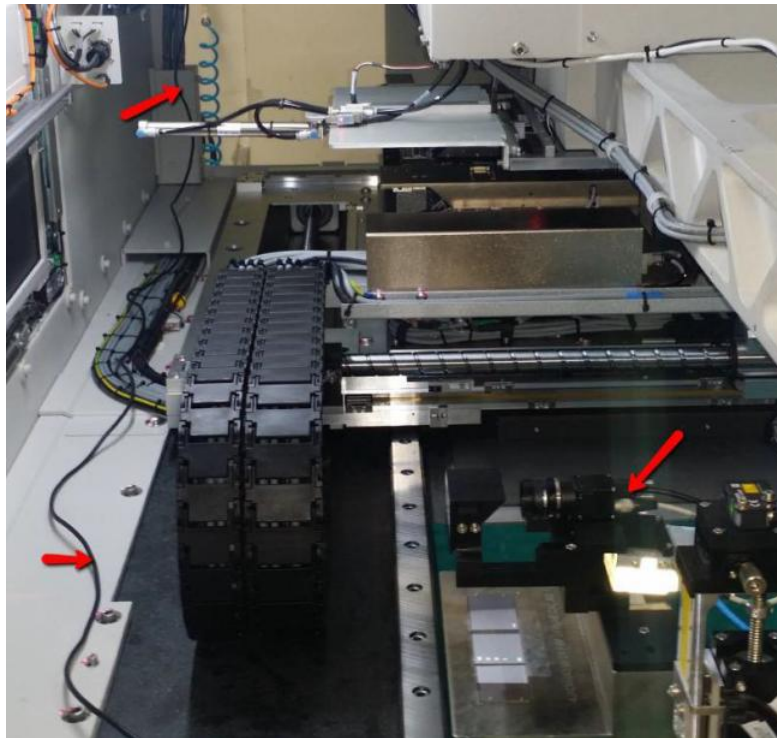
Figure 9 Camera Cable Routing (Reference Only)
