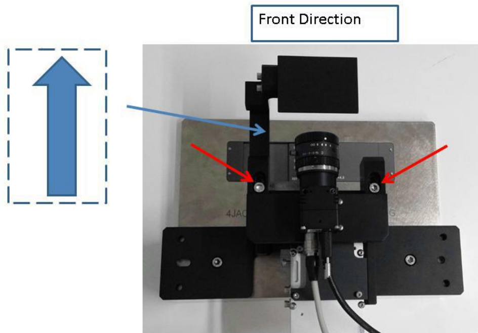
Figure 36 Module Extend towards Front Direction
